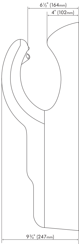
SIDE ELEVATION
